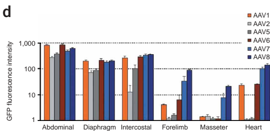
Figure 1 Systemic gene delivery to muscle and heart of neonatal mice by different AAV serotypes via i.p. injection. (a) Whole-body fluorescent photography of 2-month-old mice after i.p. injection of 2 \times 10^{11} v.g. of various dsAAV-CB-GFP at 1 d old. Note the widespread GFP expression in the foreleg, back and shoulder muscles in mice treated with AAV7 and AAV8. (b) Time course of GFP gene expression in mice after i.p. injection of 2 \times 10^{11} v.g. of dsAAV8-CB-GFP at 6 d old. (c) GFP expression seen in cryosections of heart, muscle and nonmuscle tissues at 2 months after neonatal i.p. injection of 2 \times 10^{11} v.g. of dsAAV8-CB-GFP. Numbers in parentheses denote microscopy exposure time in seconds (s). Note strong GFP expression in heart and muscles, and minimal to undetectable GFP expression in nonmuscle tissues. Scale bar, 100 \mu m. (d) Quantification of GFP fluorescence in muscle and heart cryosections of mice, which were injected i.p. with 2 \times 10^{11} v.g. of various serotypes of dsAAV-CB-GFP vectors at neonatal age. Analysis was done 2 months after gene delivery.
